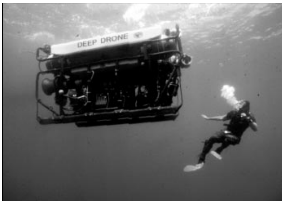
Figure 13-2. Remotely Operated Vehicle (ROV) Deep Drone.
