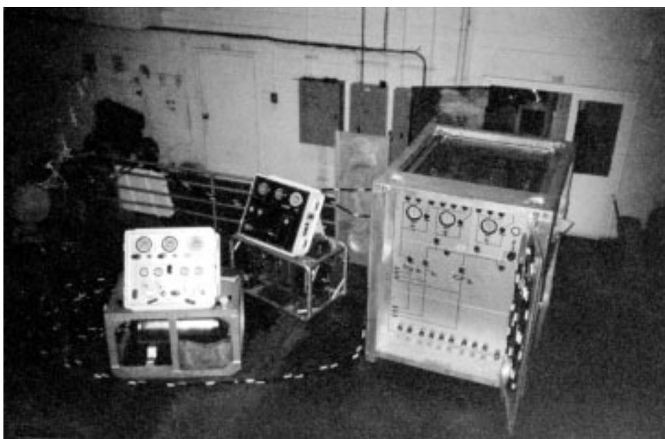
Figure 8-6. Flyaway Dive System (FADS) III.
