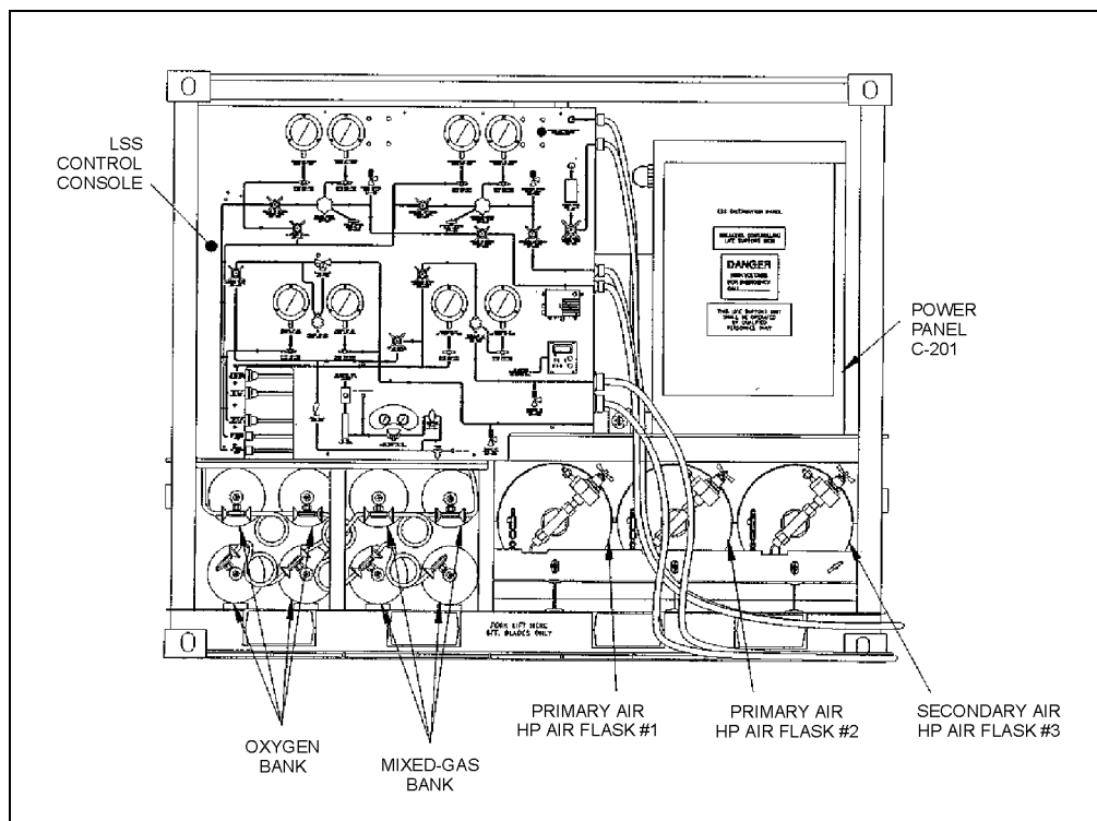
Figure 22-10. Fly Away Recompression Chamber Life Support Skid.
